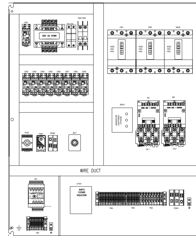
BACK PLATE
