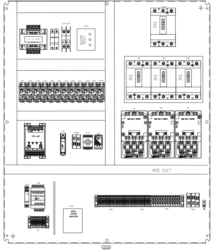
ACC00605 BACK PLATE
