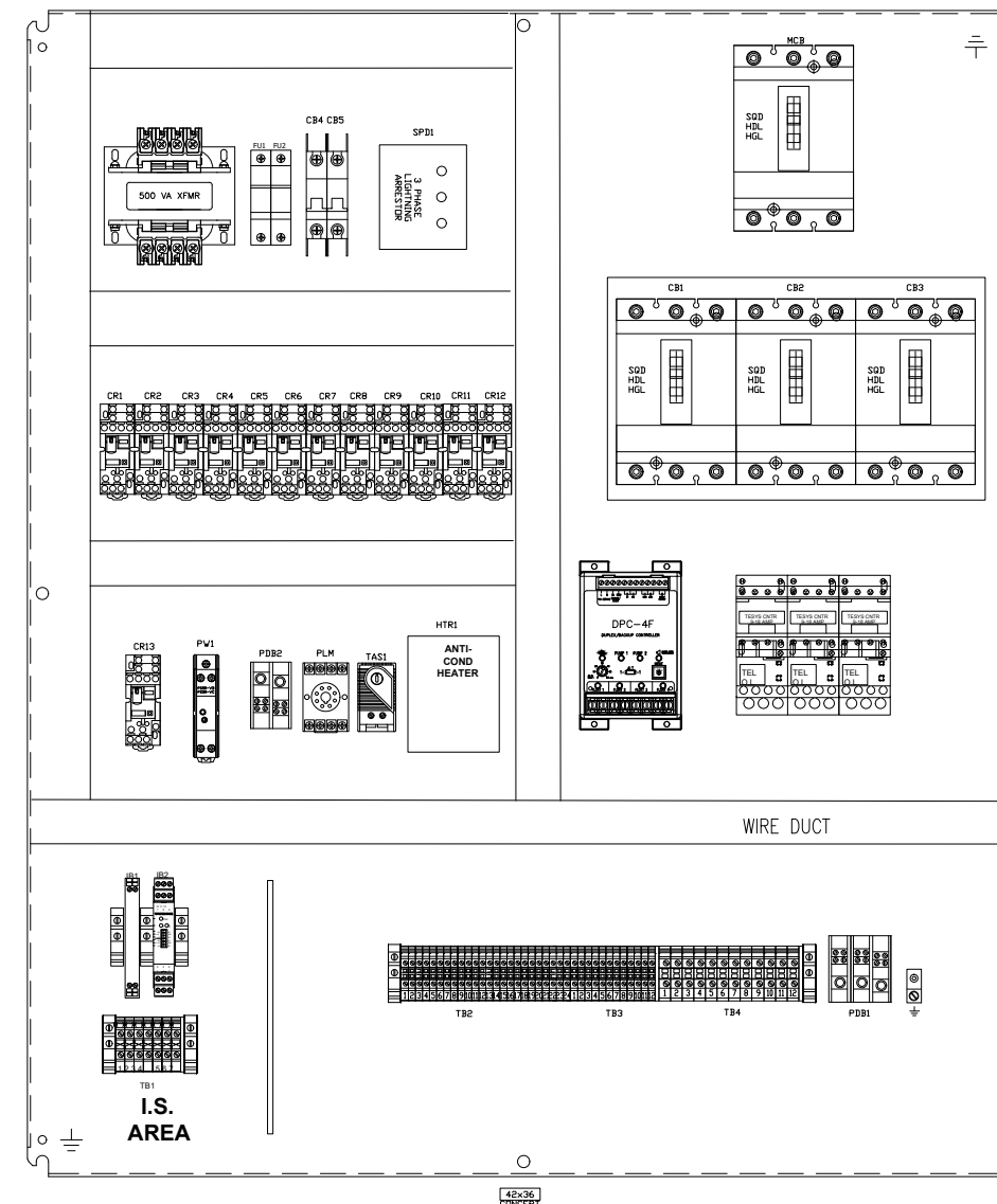
ACC00605 BACK PLATE
